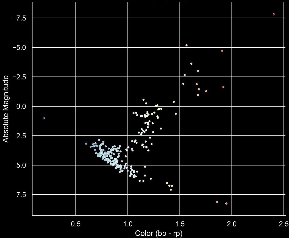
GALAH Hertzsprung-Russel Diagram Field [88] Ra [8.68] Dec [-73.55]
