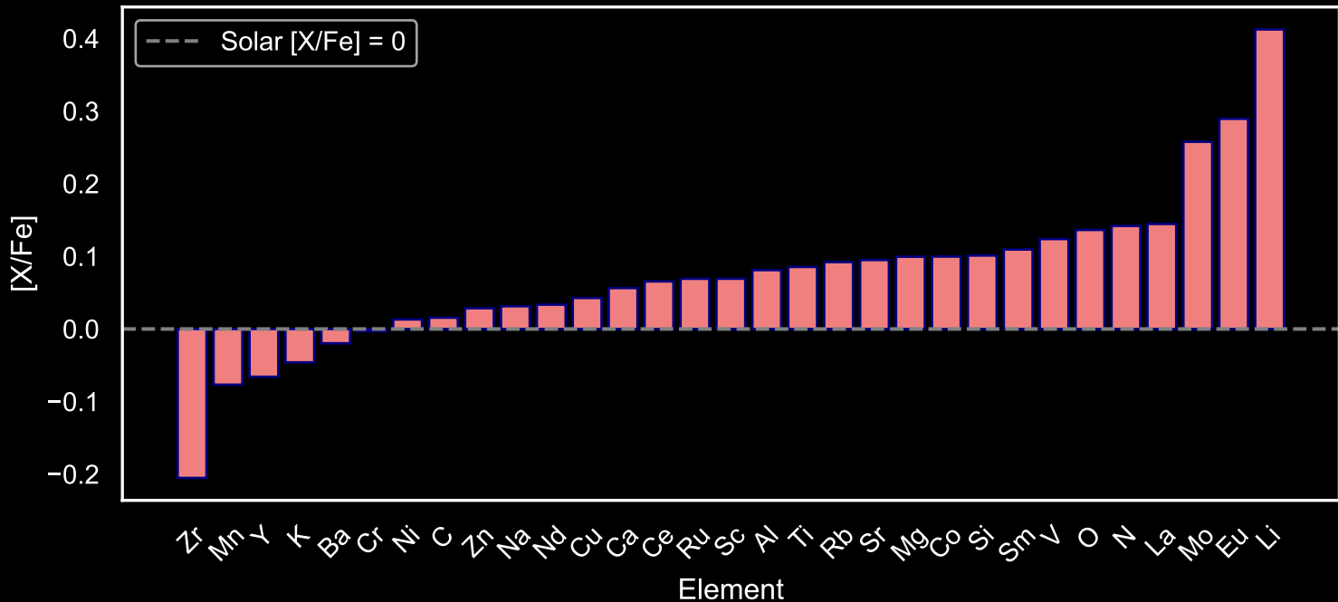
Abundance Pattern for GALAH Star Field [88] (N=241)
