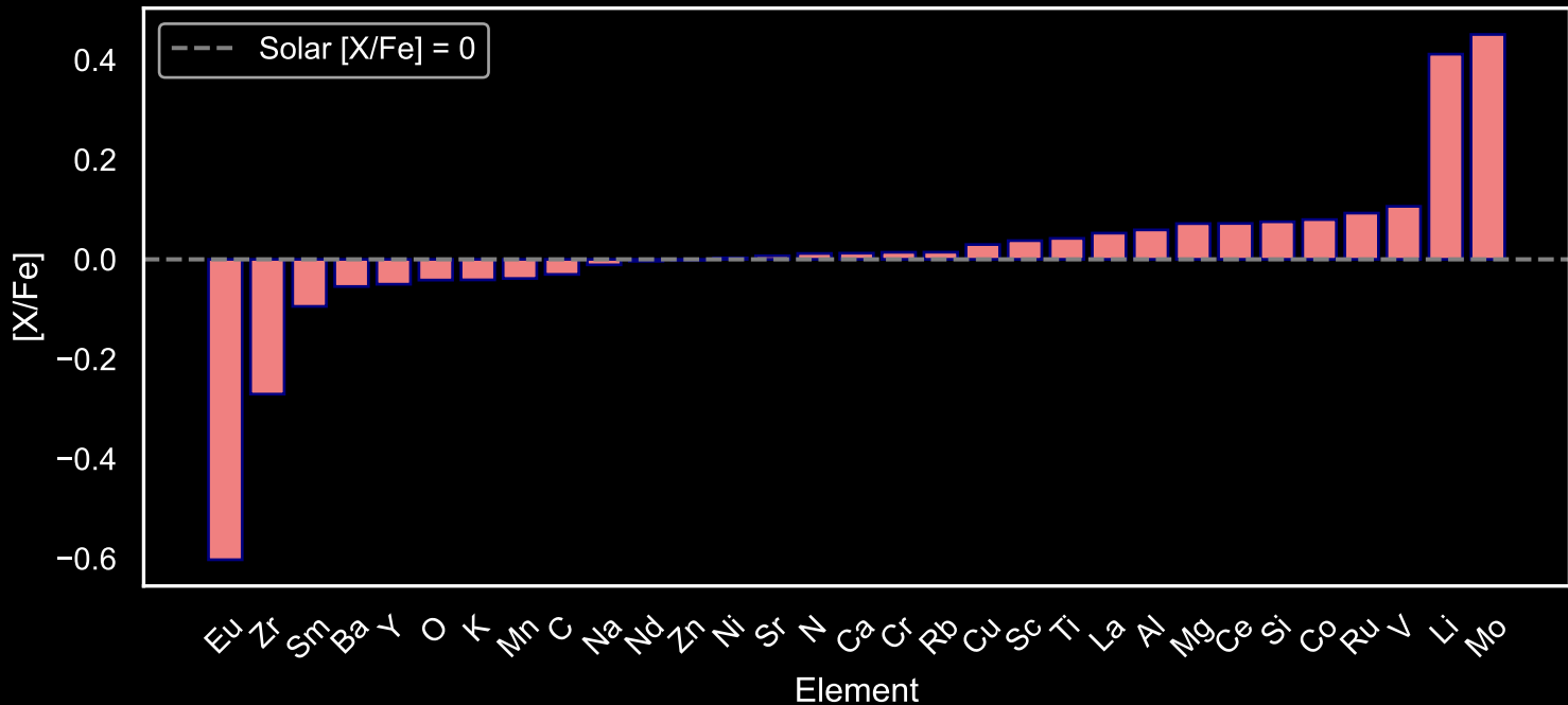
Abundance Pattern for GALAH Main Sequence Stars: Star Field [88] (N=106)
