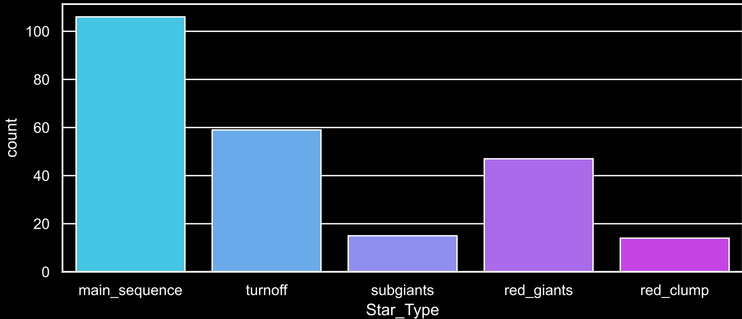
Field [88] Count plot of Star Type
