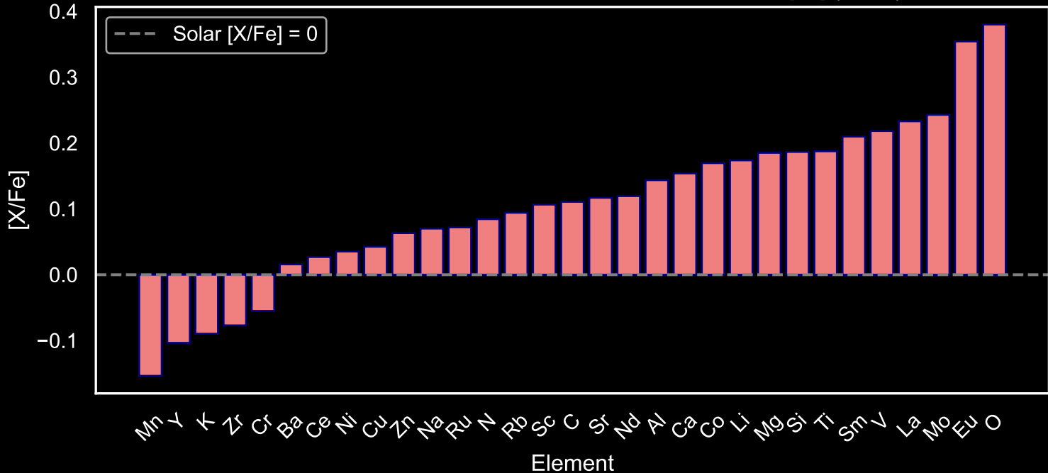
Abundance Pattern for GALAH Red Giants: Star Field [88] (N=61)
